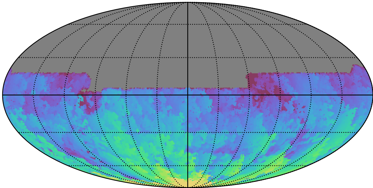
early_ss_template_fpextra2.0_v3.4_10yrs All sky u band: Max HA
