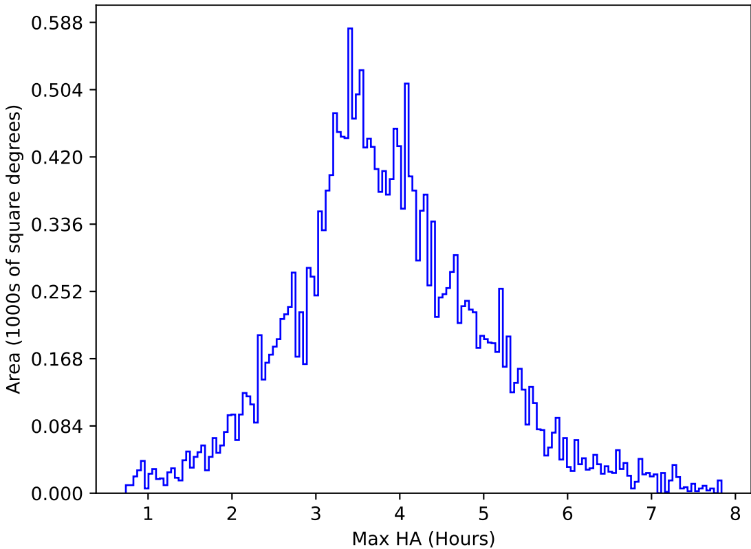
early_ss_template_fpextra2.0_v3.4_10yrs All sky u band: Max HA
