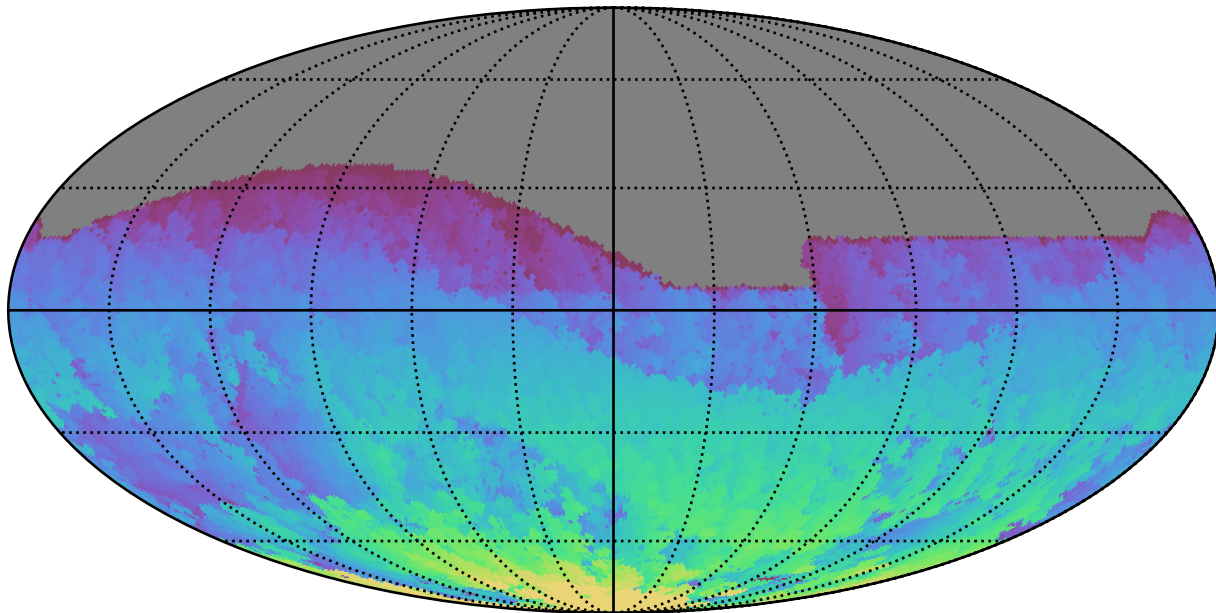
early_ss_template_fpextra2.0_v3.4_10yrs All sky i band: Max HA
