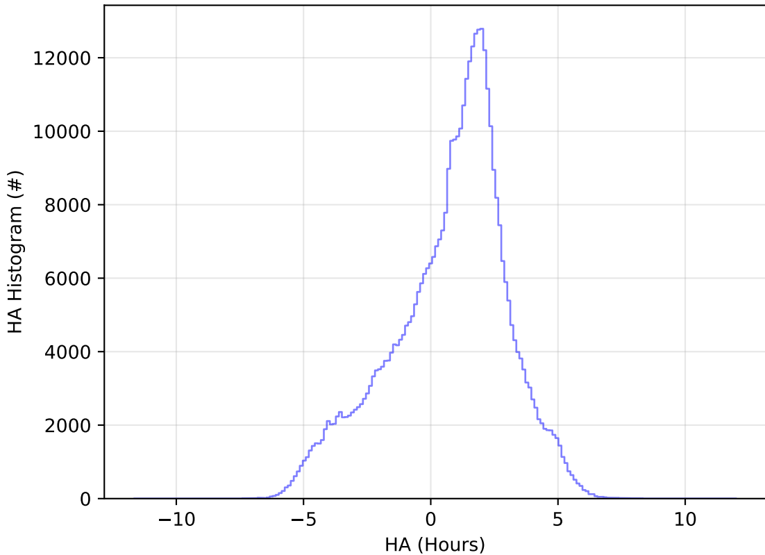
early_ss_template_fpextra2.0_v3.4_10yrs WFD z band: HA Histogram
