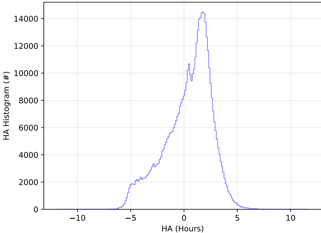
early_ss_template_fpextra2.0_v3.4_10yrs WFD r band: HA Histogram
