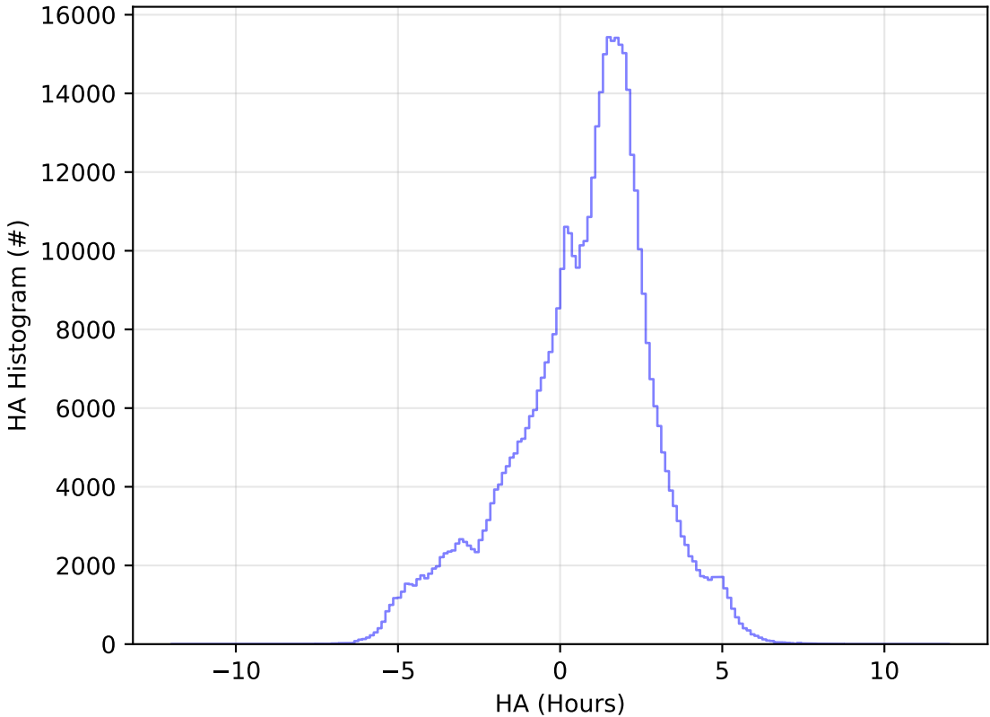
early_ss_template_fpextra2.0_v3.4_10yrs WFD i band: HA Histogram
