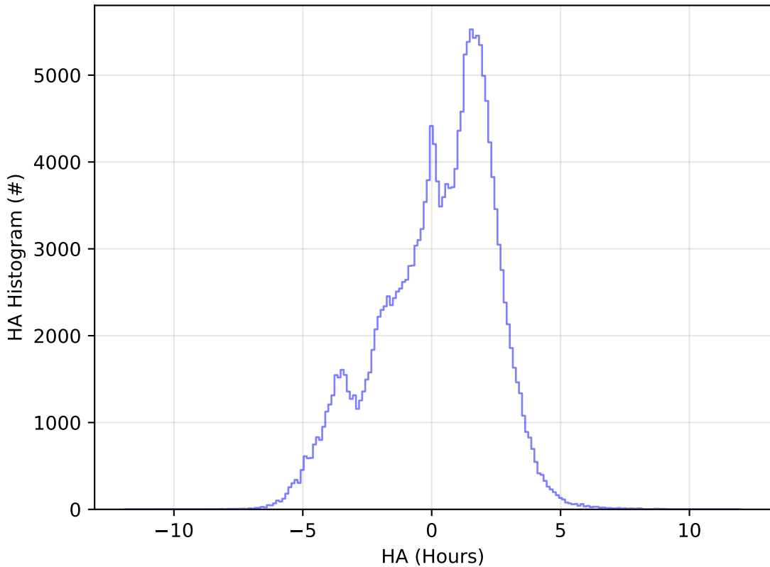
early_ss_template_fpextra2.0_v3.4_10yrs WFD g band: HA Histogram
