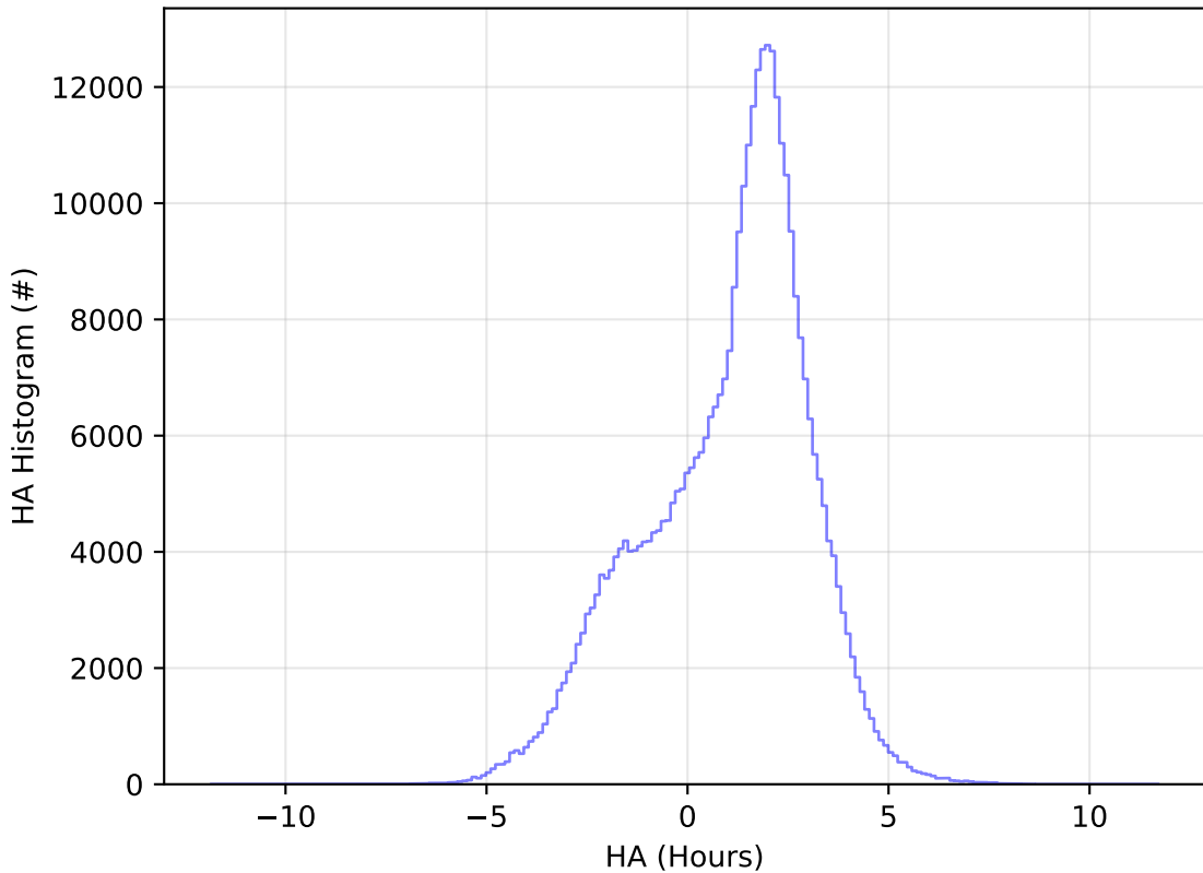
early_ss_template_fpextra2.0_v3.4_10yrs All sky y band: HA Histogram
