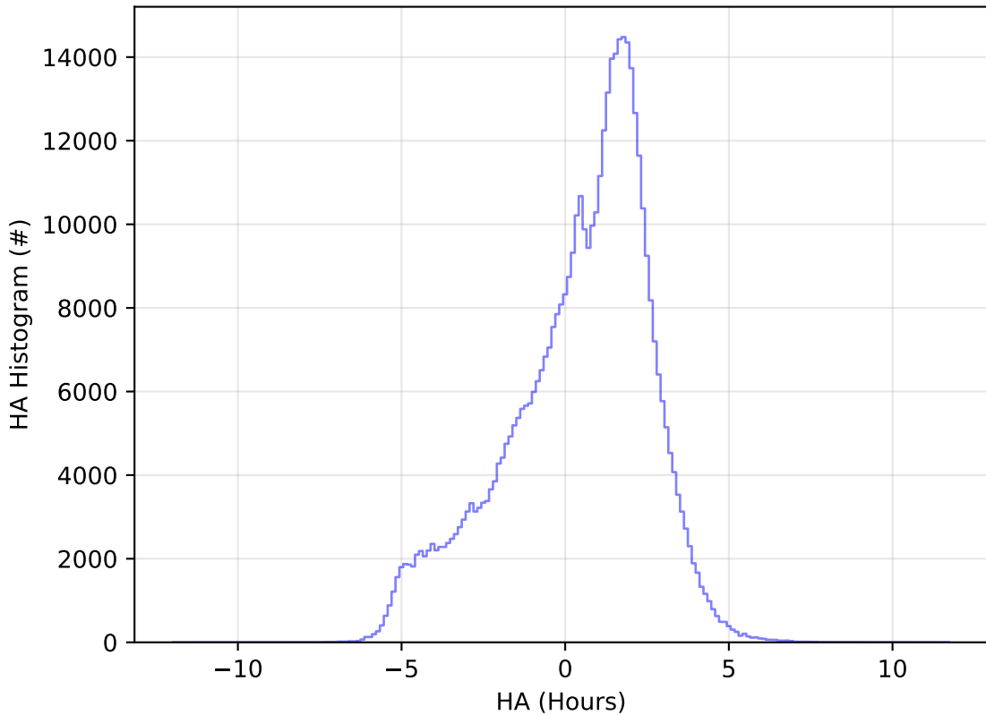
early_ss_template_fpextra2.0_v3.4_10yrs All sky r band: HA Histogram
