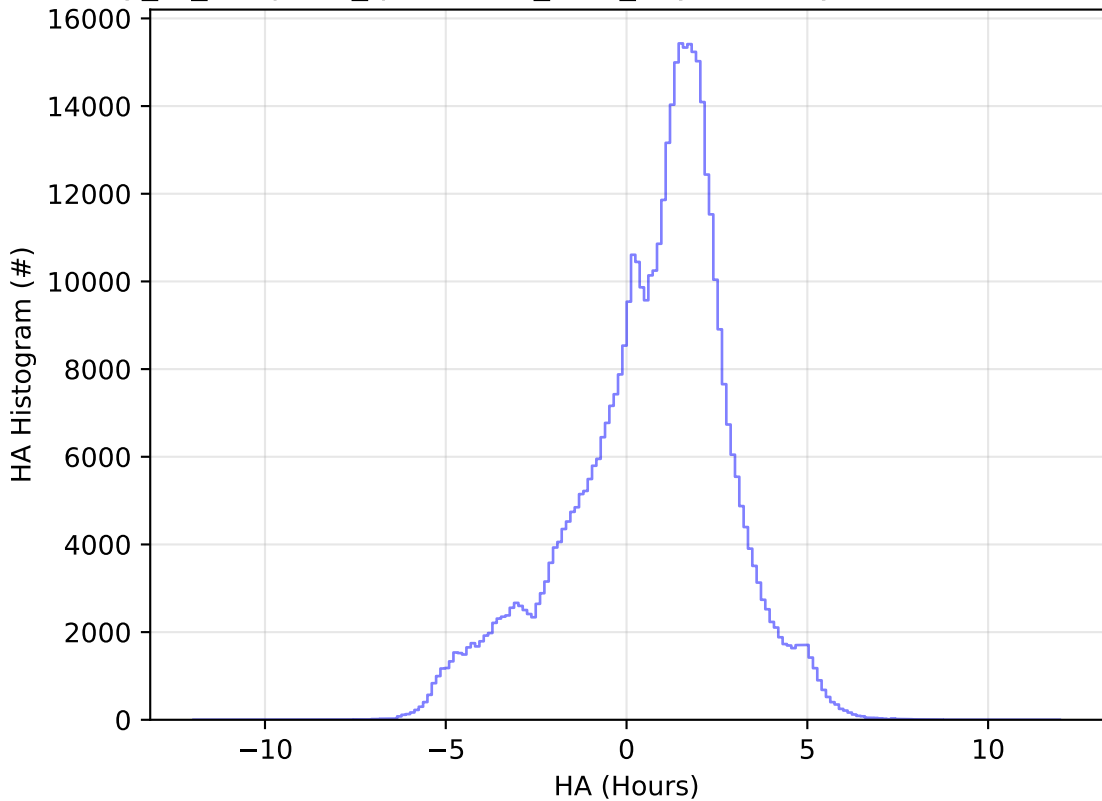
early_ss_template_fpextra2.0_v3.4_10yrs All sky i band: HA Histogram
