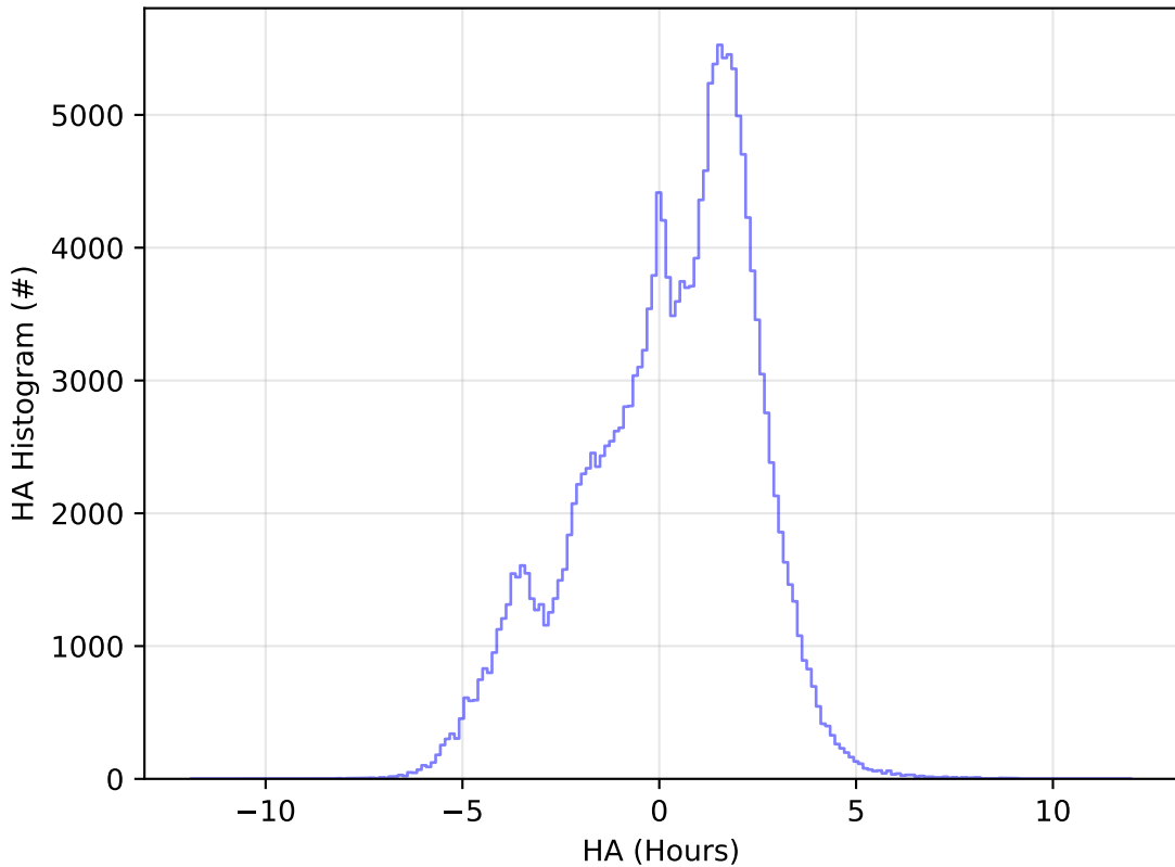
early_ss_template_fpextra2.0_v3.4_10yrs All sky g band: HA Histogram
