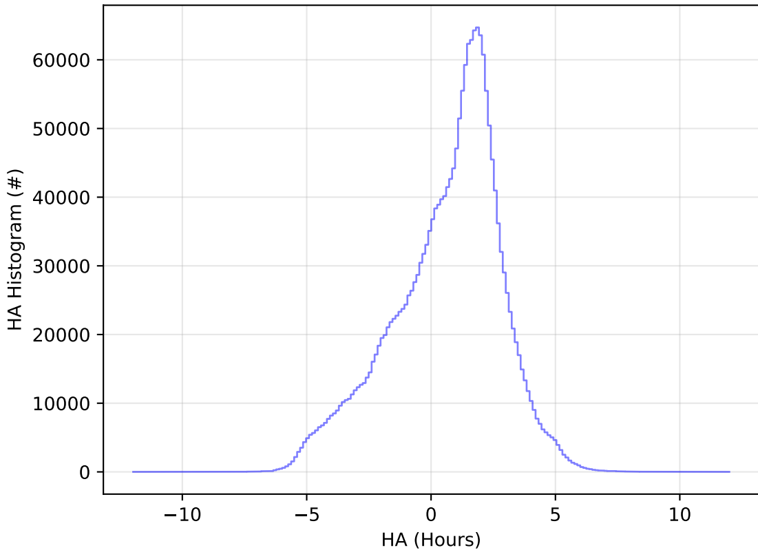
early_ss_template_fpextra2.0_v3.4_10yrs All sky all bands: HA Histogram
