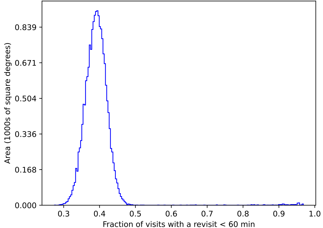
early_ss_template_fpextra2.0_v3.4_10yrs gri WFD: Fraction of visits with a revisit < 60 min
