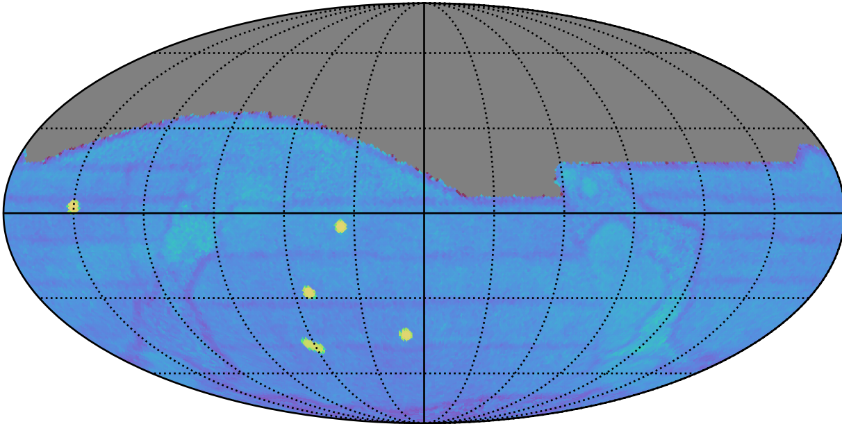
early_ss_template_fpextra2.0_v3.4_10yrs gri All sky: Fraction of visits with a revisit < 60 min
