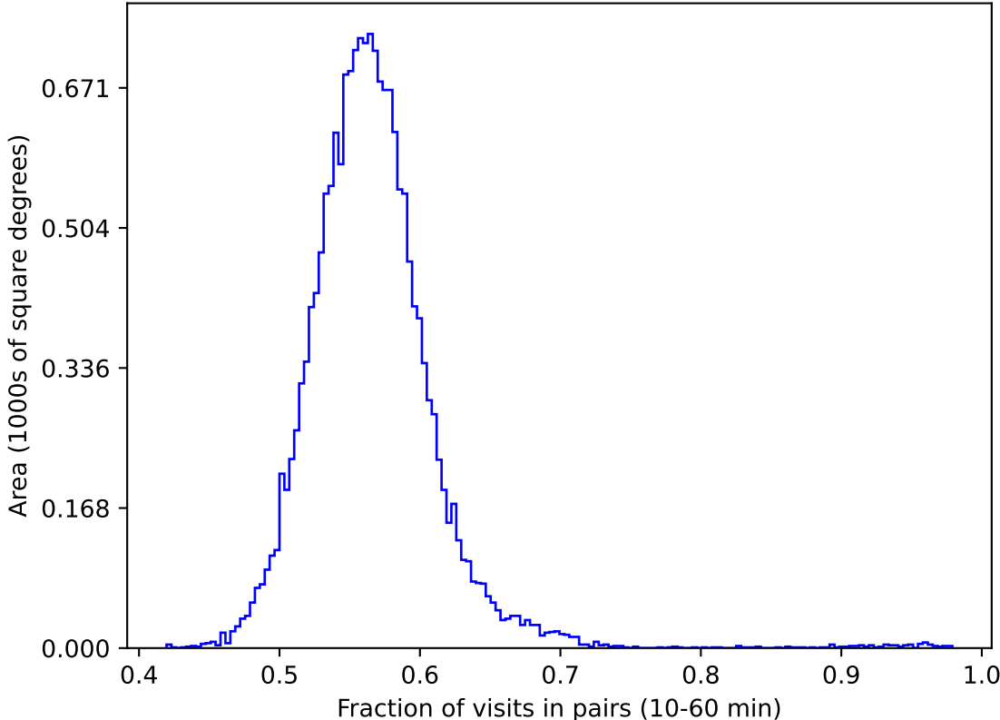
early_ss_template_fpextra2.0_v3.4_10yrs gri WFD: Fraction of visits in pairs (10-60 min)
