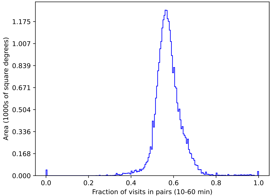
early_ss_template_fpextra2.0_v3.4_10yrs gri All sky: Fraction of visits in pairs (10-60 min)
