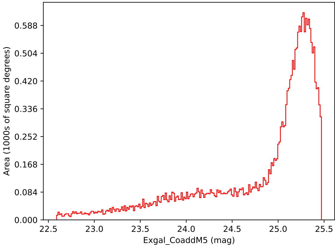
early_ss_template_fpextra2.0_v3.4_10yrs Yr 1 i band: Exgal_CoaddM5
