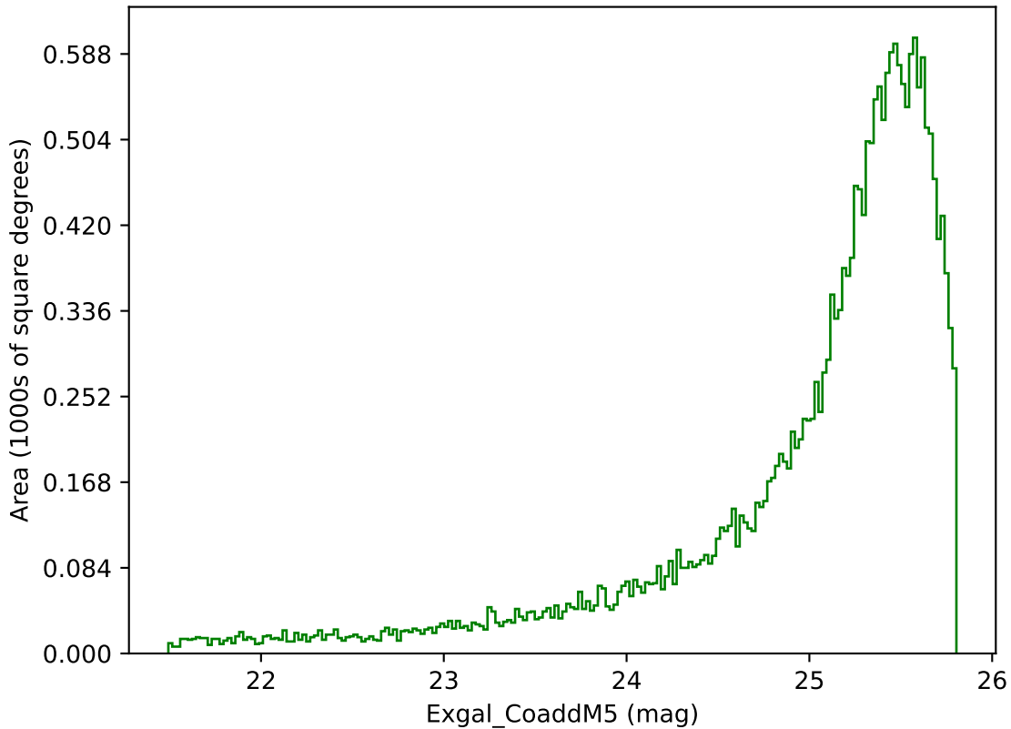
early_ss_template_fpextra2.0_v3.4_10yrs Yr 1 g band: Exgal_CoaddM5
