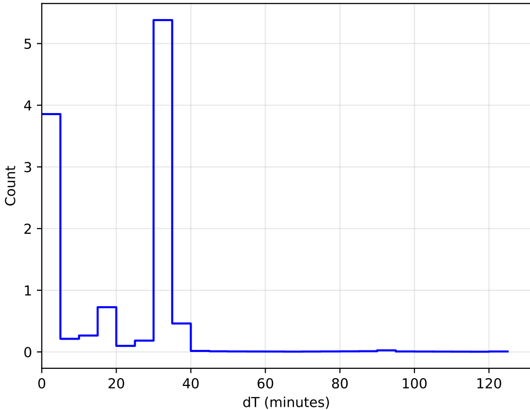
early_ss_template_fpextra2.0_v3.4_10yrs WFD: DeltaT Histogram
