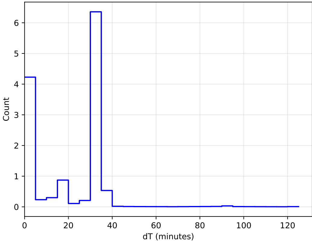
early_ss_template_fpextra2.0_v3.4_10yrs All sky: DeltaT Histogram
