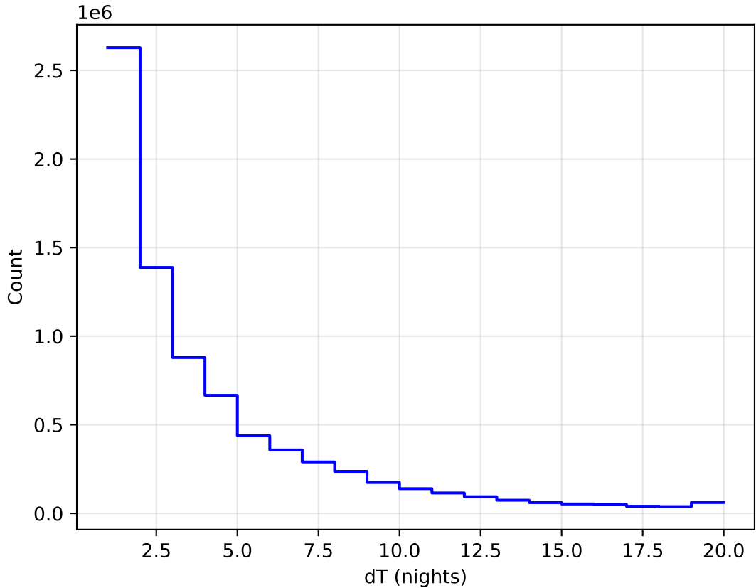
early_ss_template_fpextra2.0_v3.4_10yrs WFD all bands: DeltaNight Histogram
