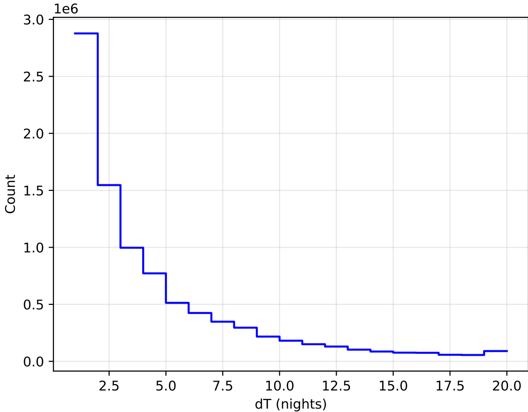
early_ss_template_fpextra2.0_v3.4_10yrs All sky all bands: DeltaNight Histogram
