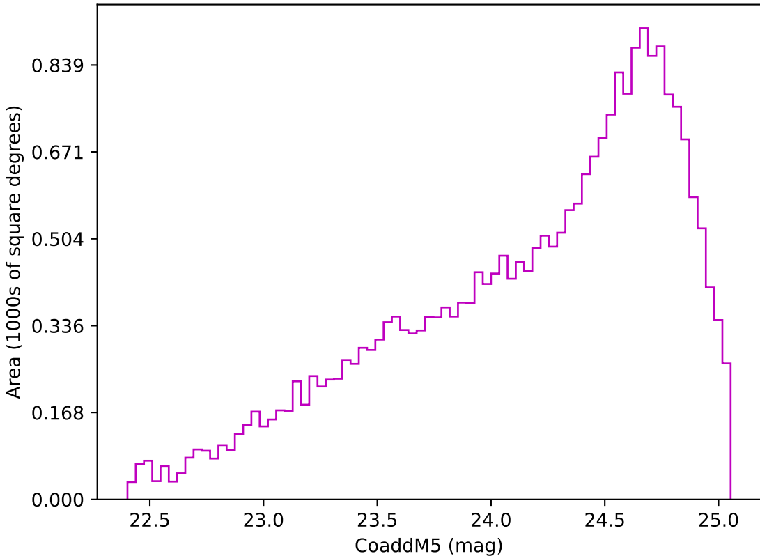
early_ss_template_fpextra2.0_v3.4_10yrs Yr 3-4 z band: CoaddM5
