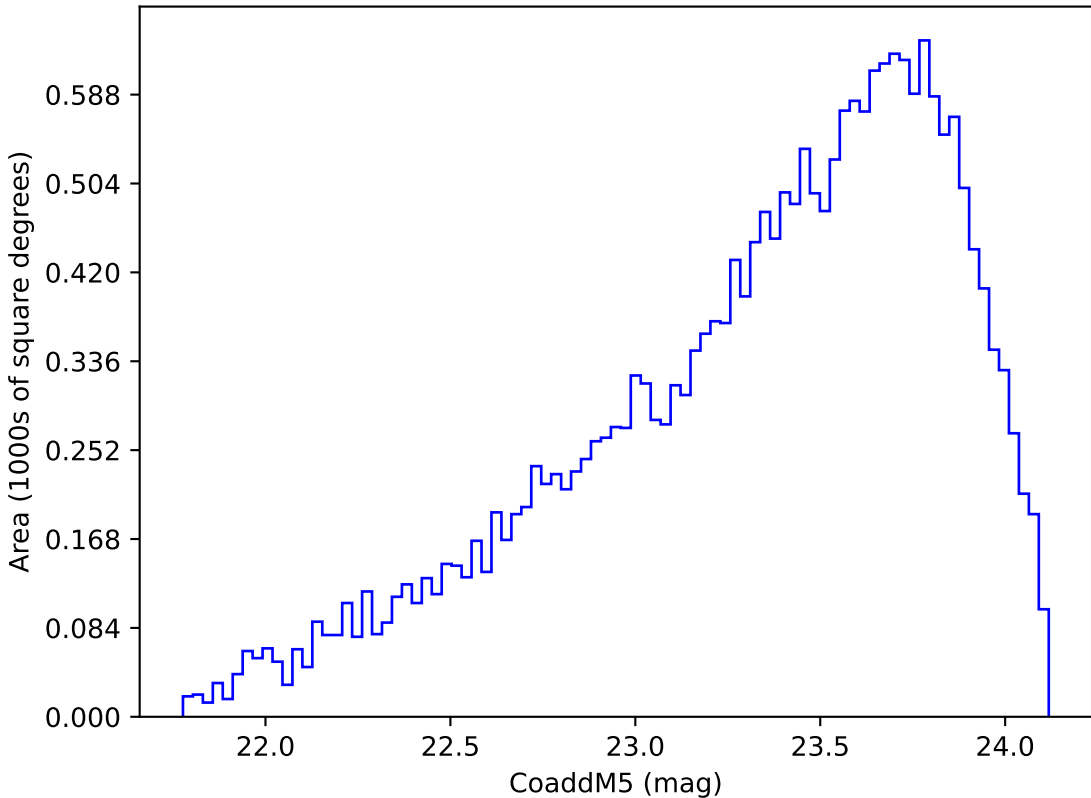
early_ss_template_fpextra2.0_v3.4_10yrs Yr 3-4 y band: CoaddM5
