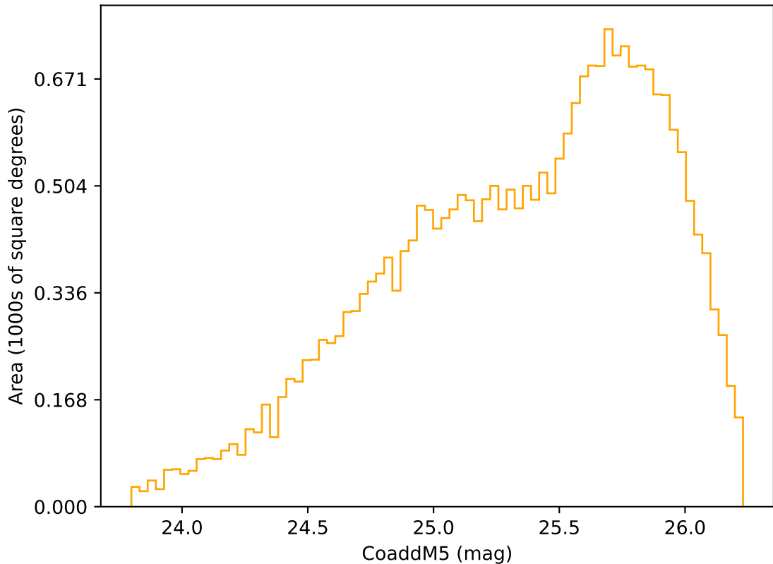
early_ss_template_fpextra2.0_v3.4_10yrs Yr 3-4 r band: CoaddM5
