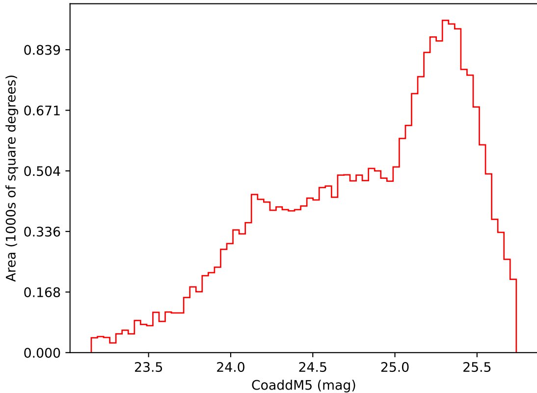
early_ss_template_fpextra2.0_v3.4_10yrs Yr 3-4 i band: CoaddM5
