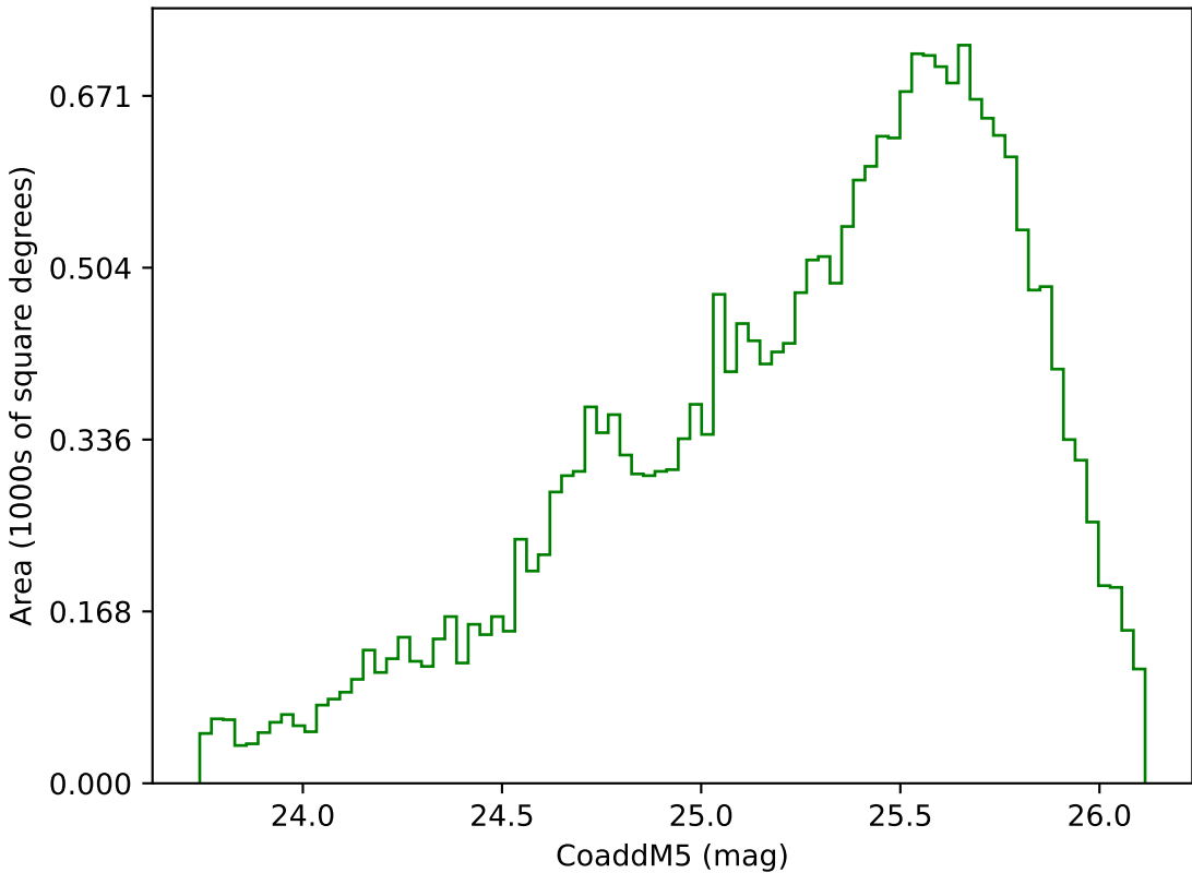
early_ss_template_fpextra2.0_v3.4_10yrs Yr 3-4 g band: CoaddM5
