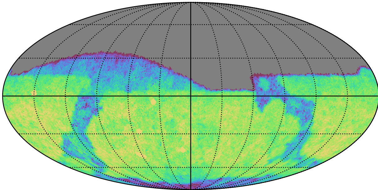
early_ss_template_fpextra2.0_v3.4_10yrs Yr 1 z band: CoaddM5
