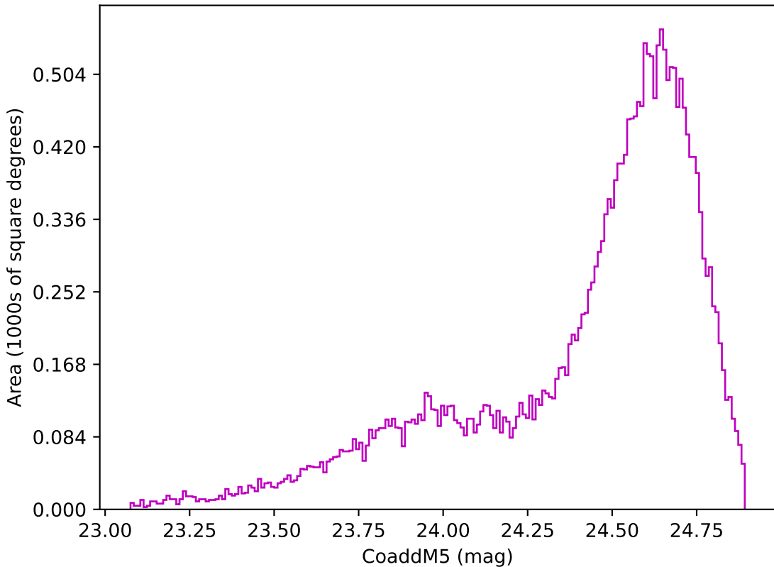
early_ss_template_fpextra2.0_v3.4_10yrs Yr 1 z band: CoaddM5
