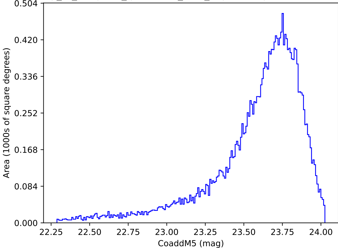
early_ss_template_fpextra2.0_v3.4_10yrs Yr 1 y band: CoaddM5
