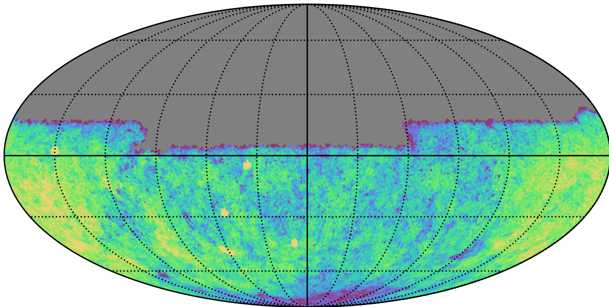
early_ss_template_fpextra2.0_v3.4_10yrs Yr 1 u band: CoaddM5
