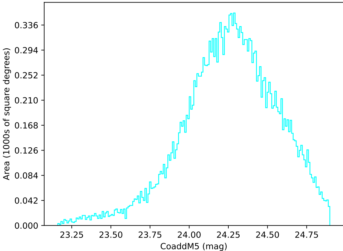
early_ss_template_fpextra2.0_v3.4_10yrs Yr 1 u band: CoaddM5
