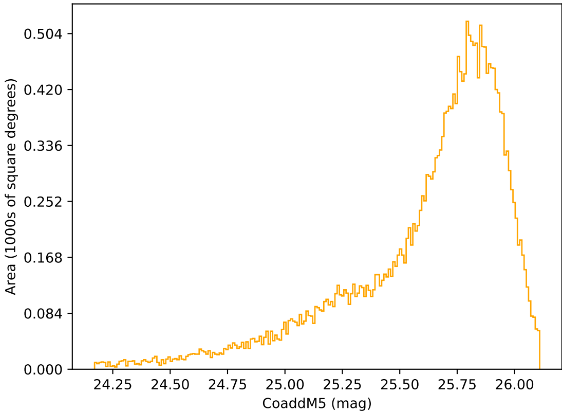
early_ss_template_fpextra2.0_v3.4_10yrs Yr 1 r band: CoaddM5
