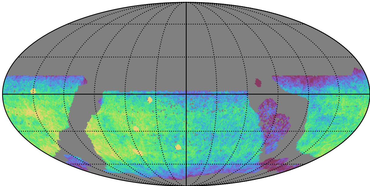
early_ss_template_fpextra2.0_v3.4_10yrs WFD u band: CoaddM5
