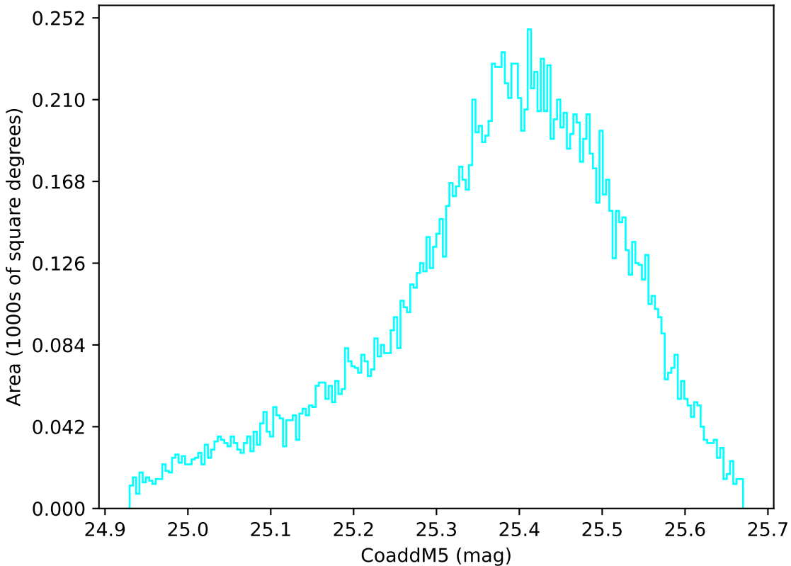
early_ss_template_fpextra2.0_v3.4_10yrs WFD u band: CoaddM5
