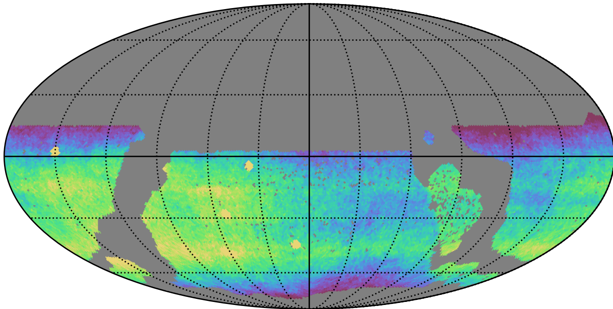
early_ss_template_fpextra2.0_v3.4_10yrs WFD r band: CoaddM5
