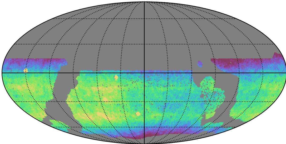
early_ss_template_fpextra2.0_v3.4_10yrs WFD i band: CoaddM5
