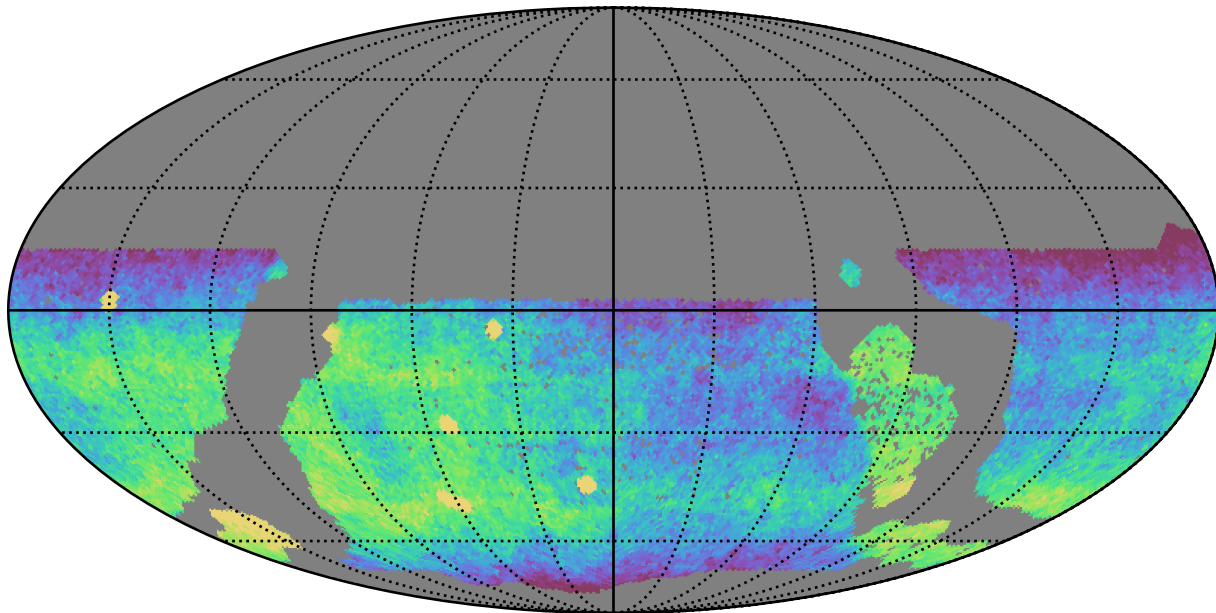
early_ss_template_fpextra2.0_v3.4_10yrs WFD g band: CoaddM5
