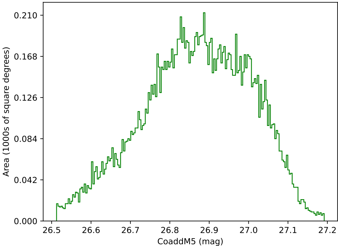
early_ss_template_fpextra2.0_v3.4_10yrs WFD g band: CoaddM5
