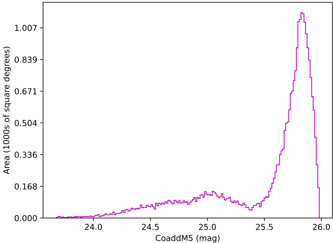
early_ss_template_fpextra2.0_v3.4_10yrs All sky z band: CoaddM5
