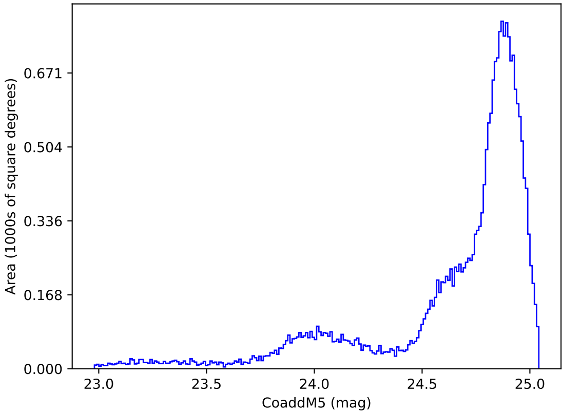
early_ss_template_fpextra2.0_v3.4_10yrs All sky y band: CoaddM5
