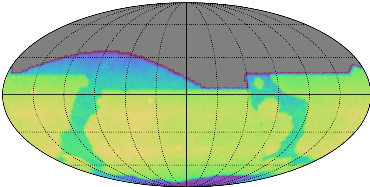
early_ss_template_fpextra2.0_v3.4_10yrs All sky i band: CoaddM5
