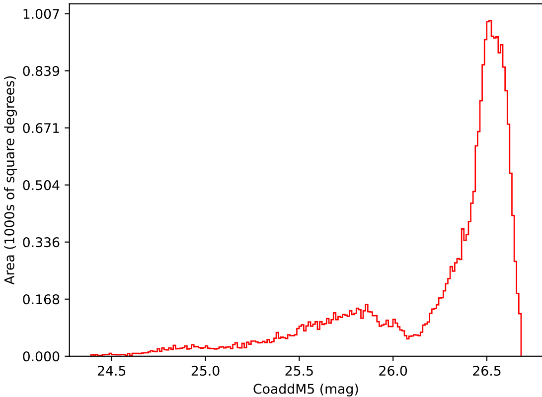
early_ss_template_fpextra2.0_v3.4_10yrs All sky i band: CoaddM5
