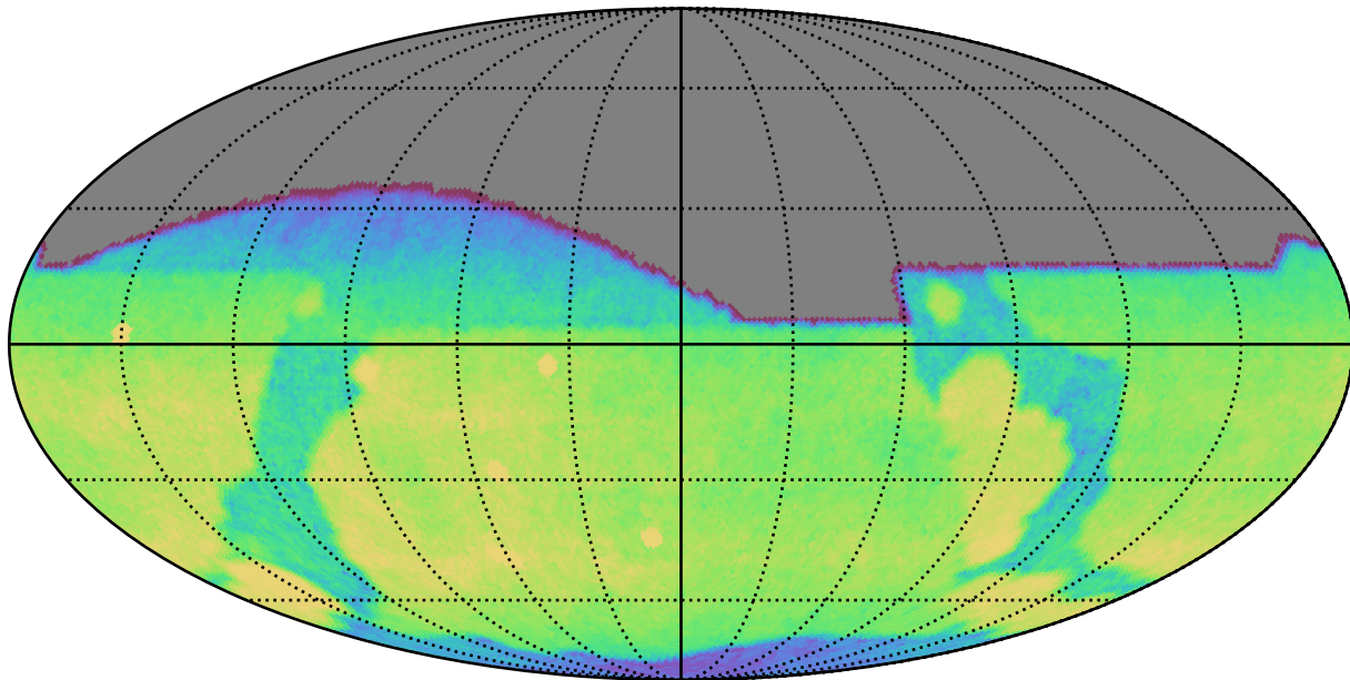
early_ss_template_fpextra2.0_v3.4_10yrs All sky g band: CoaddM5
