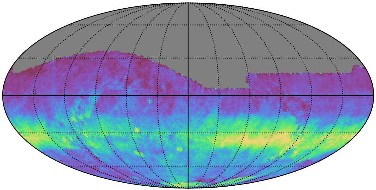
early_ss_template_fpextra2.0_v3.4_10yrs All sky r band: AngleRms rotSkyPos
