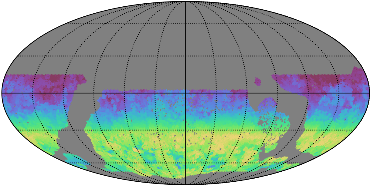
early_ss_template_fpextra2.0_v3.4_10yrs WFD z band: AngleRange rotSkyPos
