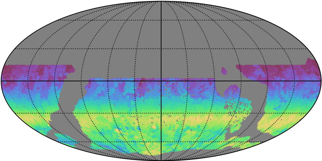
early_ss_template_fpextra2.0_v3.4_10yrs WFD r band: AngleRange rotSkyPos
