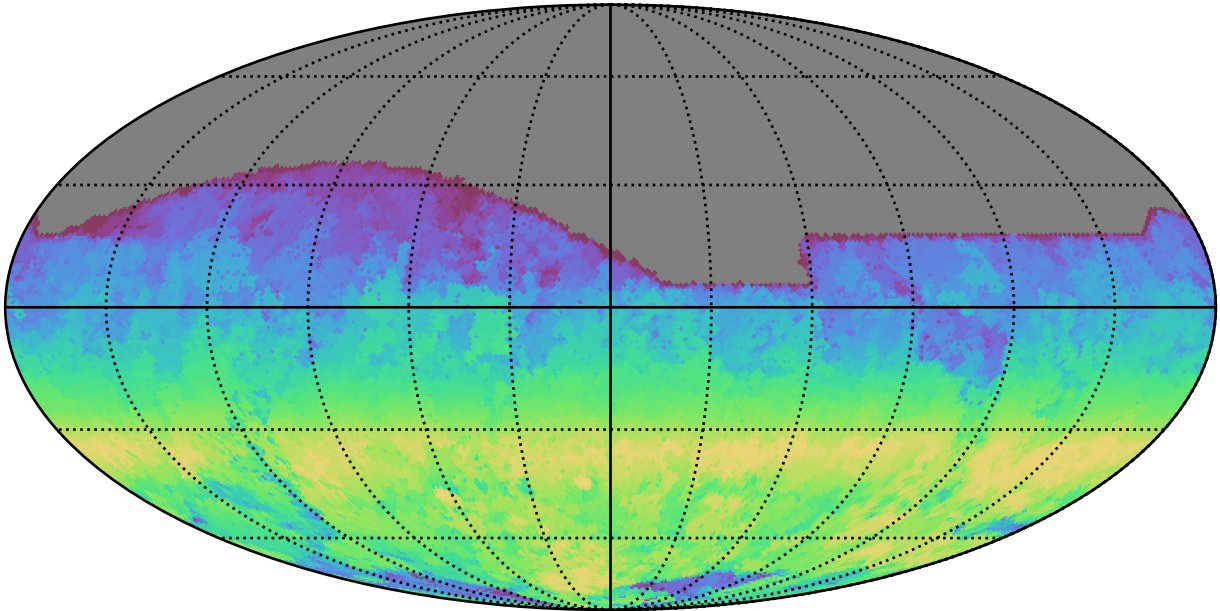
early_ss_template_fpextra2.0_v3.4_10yrs All sky r band: AngleRange rotSkyPos
