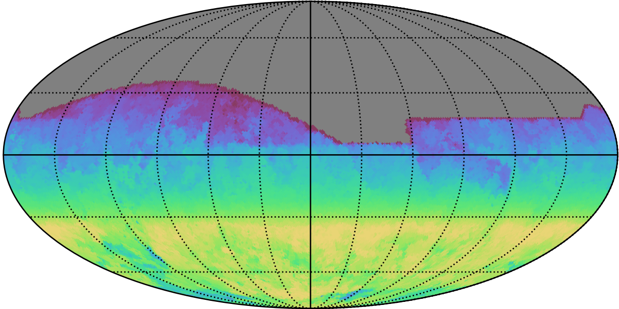
early_ss_template_fpextra2.0_v3.4_10yrs All sky all bands: AngleRange rotSkyPos
