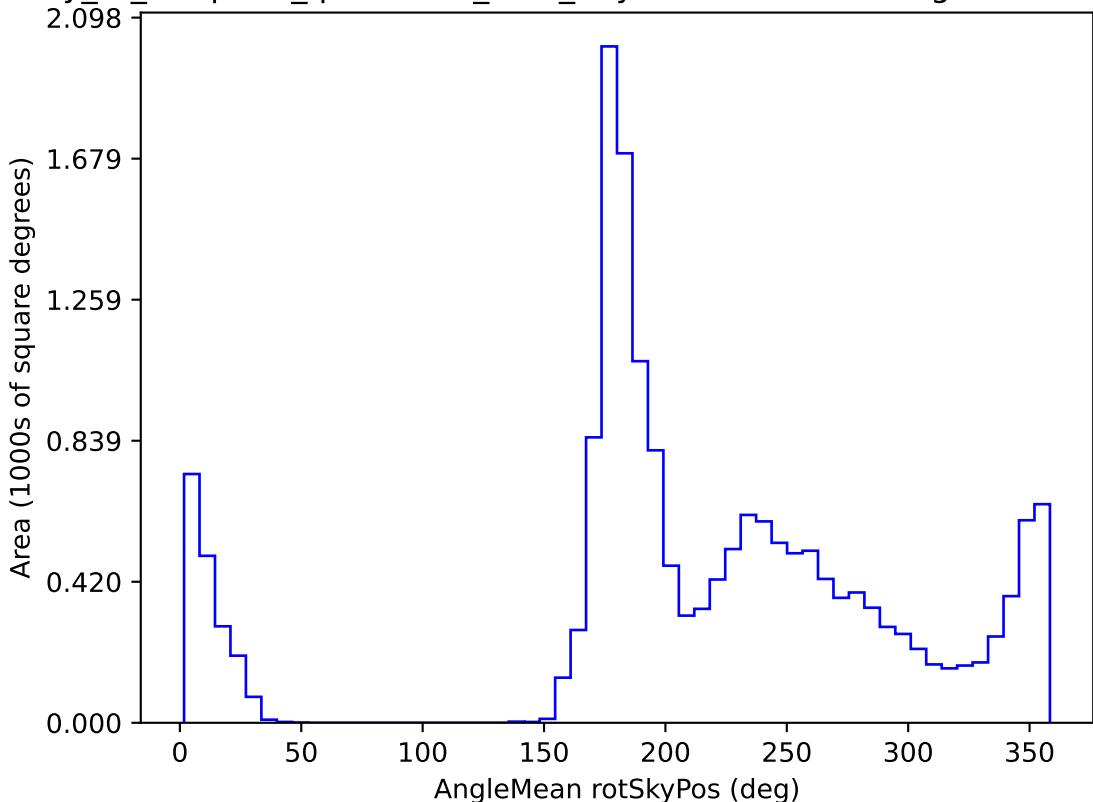
early_ss_template_fpextra2.0_v3.4_10yrs WFD z band: AngleMean rotSkyPos
